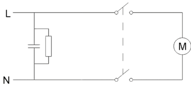
Schematic Diagram
